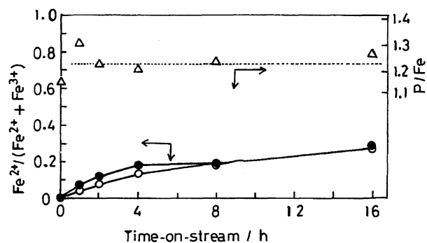
Fig. 5. Variation in P/Fe and Fe 2+ /(Fe 2+ + Fe 3+ ) ratios as a function of the time of IBA oxidation. (O) in the bulk; (●) on the surface. Sample: freshly prepared iron phosphate. Reaction temperature: 380 °C.
