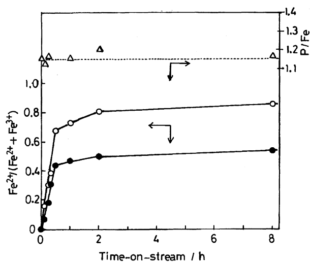
Fig. 6. Variation in P/Fe and Fe 2+ /(Fe 2+ + Fe 3+ ) ratios as a function of the reduction time. (O) in the bulk; (●) on the surface. Feed gas rates: IBA/H 2 O/N 2 = 21.5/324/350 mmol h -1 . Sample: freshly prepared iron phosphate. Reduction temperature: 380 °C.
